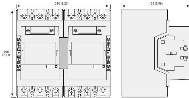
Figure 82 - 104-E190, 104-E205 Reversing Contactors with Cat. No. 100-EM... Mechanical Interlock
