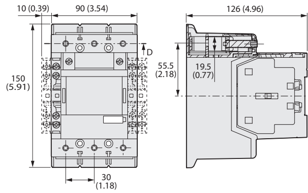
Figure 77 - 100-E116E..., 100-E146E... Contactors with PLC Input
